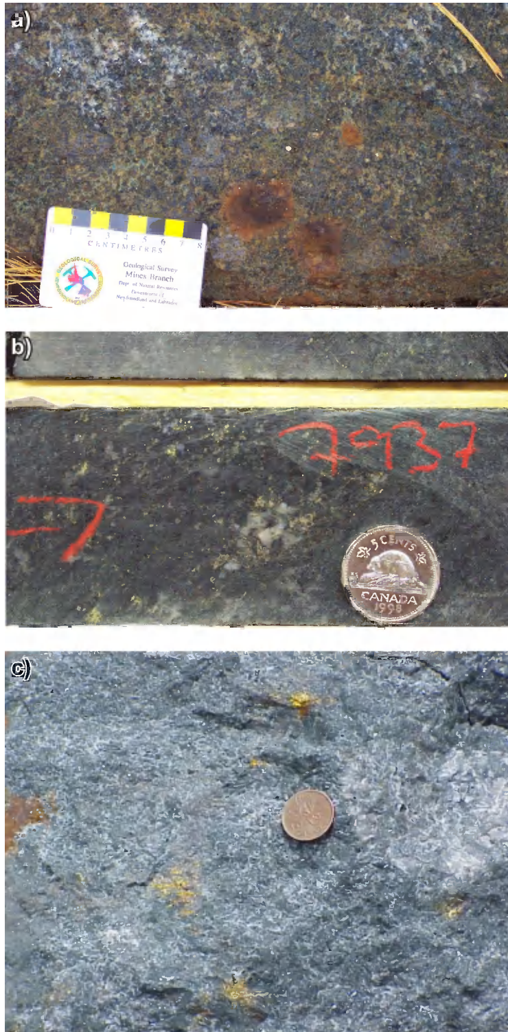
Frontispiece. Typical copper-nickel-PGE mineralization from the River Valley intrusion. a) Typical outcrop exposure of mineralized olivine gabbro-norite from the River Valley intrusion in the vicinity of the Jackson's Flats occurrence. Note sulphide "burns" to the right of the 8.5 cm long scale card. b) Drill core from drill hole DL-14 in the Dana North area (Stop 9C, Day 3), showing the typical low tenor of sulphide and the presence of blue-grey quartz. A sample like this typically contains greater than 2 g/t of Pt and Pd mineralization. c) Close-up of mineralization from the Inclusion-Bearing unit at Dana South (Stop 9F, Day 3). All photographs courtesy of S. Jobin-Bevans.
