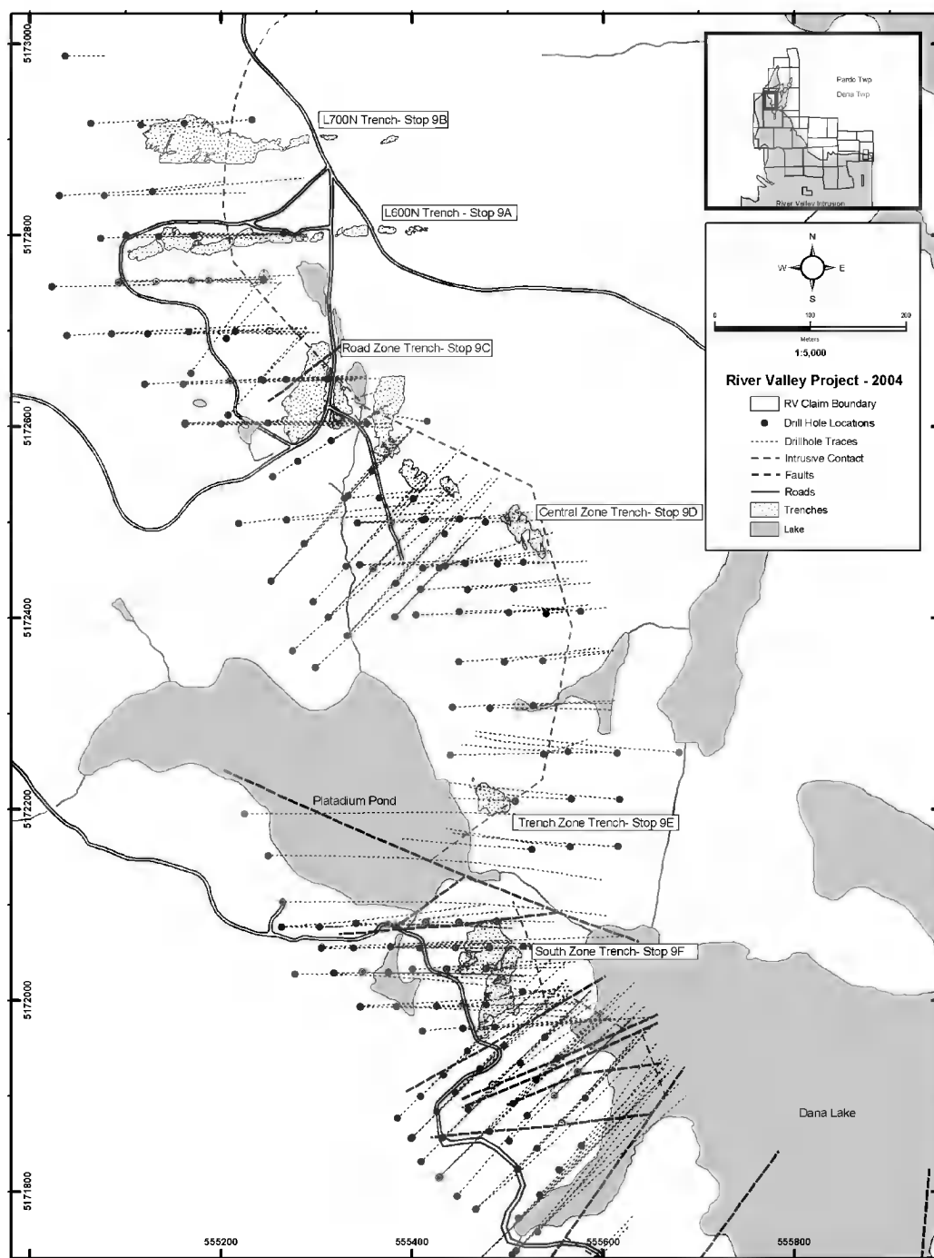
Figure 12. Map of the Dana North property of Pacific North West Capital Corporation, showing the location of stops 9A through 9F, as well as the extent of the drilling program undertaken between 1999 and 2002.
