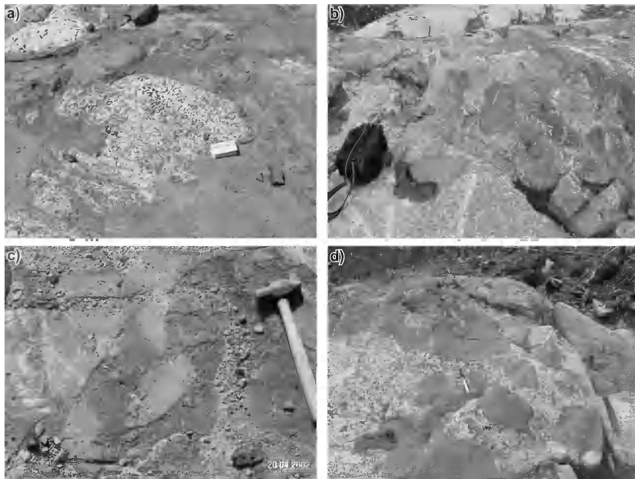
Photo 13. Photographs illustrating the textural variation observed in the Inclusion-Bearing unit in the Dana North area (Day 3, Stop 9). a) Large, leucogabbronorite fragment hosted in a gabbronorite to pyroxenite matrix. Scale card is approximately 8.5 cm long. b) Gabbronorite to pyroxenite fragments hosted in a leucogabbronorite matrix in stripped outcrop at the central zone (stop 9D, Day 3). c) Mafic fragment and matrix-dominated portion of the Inclusion-Bearing unit at Dana South (stop 9F, Day 3). Hammer handle is approximately 35 cm long. d) Gabbronorite to pyroxenite fragments hosted in a leucogabbronorite matrix in stripped outcrop at the Central zone (stop 9D, Day 3). Marker is approximately 14 cm long.
