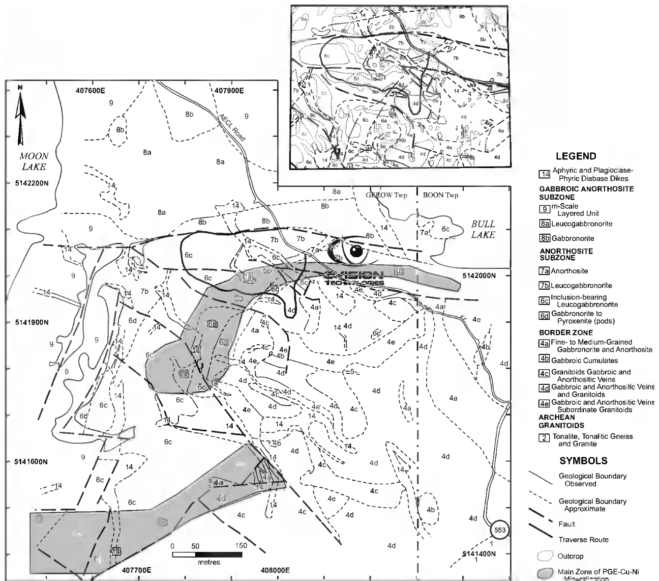
Figure 6. Geological map of the Moon Lake area, East Bull Lake Intrusion, showing the route of the traverse (heavy line) undertaken during Stop 11. Shaded areas indicate areas of disseminated sulphide mineralization. D.C. Peck and P.C. Chubb originally prepared the map in 1991 for the Department of Earth Sciences, Laurentian University. Inset map in the upper right indicates in detail the route of the traverse, as well as outcrop areas crossed during the traverse. Numerical rock codes in the legend correspond to those used in Figures 2 and 3, and on the map of Chubb, Hannila and Peck (1994). Note that UTM co-ordinates in this figure are in Zone 17, datum NAD 27.
