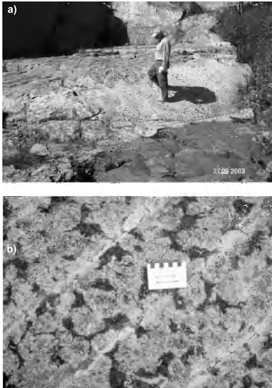
Photo 7. Stop 2, Day 2. a) Stone quarry in Nodular Anorthosite unit. Author R.S. James is standing on nodular anorthosite; dark rocks in foreground belong to a Matachewan swarm diabase dike that intrudes the Nodular Anorthosite unit. b) Close-up of nodular anorthosite, showing closely packed plagioclase glomerophenocrysts with minor interstitial, altered, pyroxene. Scale card is 8.5 cm long.
