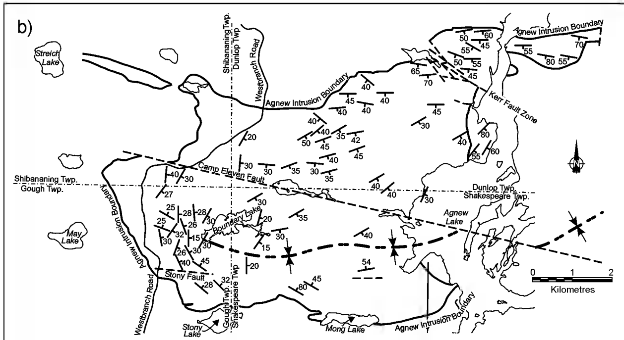
Figure 7. Geology of the Agnew Lake Intrusion. a) Geologic map showing main stratigraphic units; unit numbers correspond to those in Figure 3 and in the text. b) Structural map showing attitude of centimetre- and metre-scale layering. The strike and plunge of the axial plane of the synclinal, lopolitic structure is the same as that in the Huronian Supergroup supracrustal rocks on the east side of Agnew Lake. Both figures modified from Vogel (1996).
