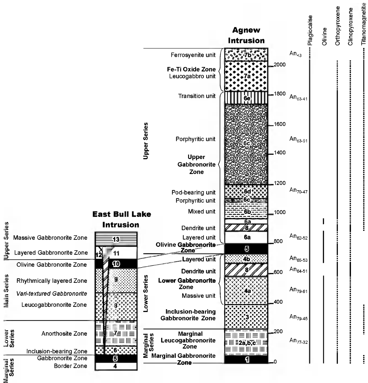
Figure 3. Stratigraphic sections for the East Bull Lake and Agnew Lake intrusions. Mineral distribution and plagioclase compositions are from Vogel et al. (1999). Unit numbers correlate with geologic maps shown in Figures 2 and 6a.
