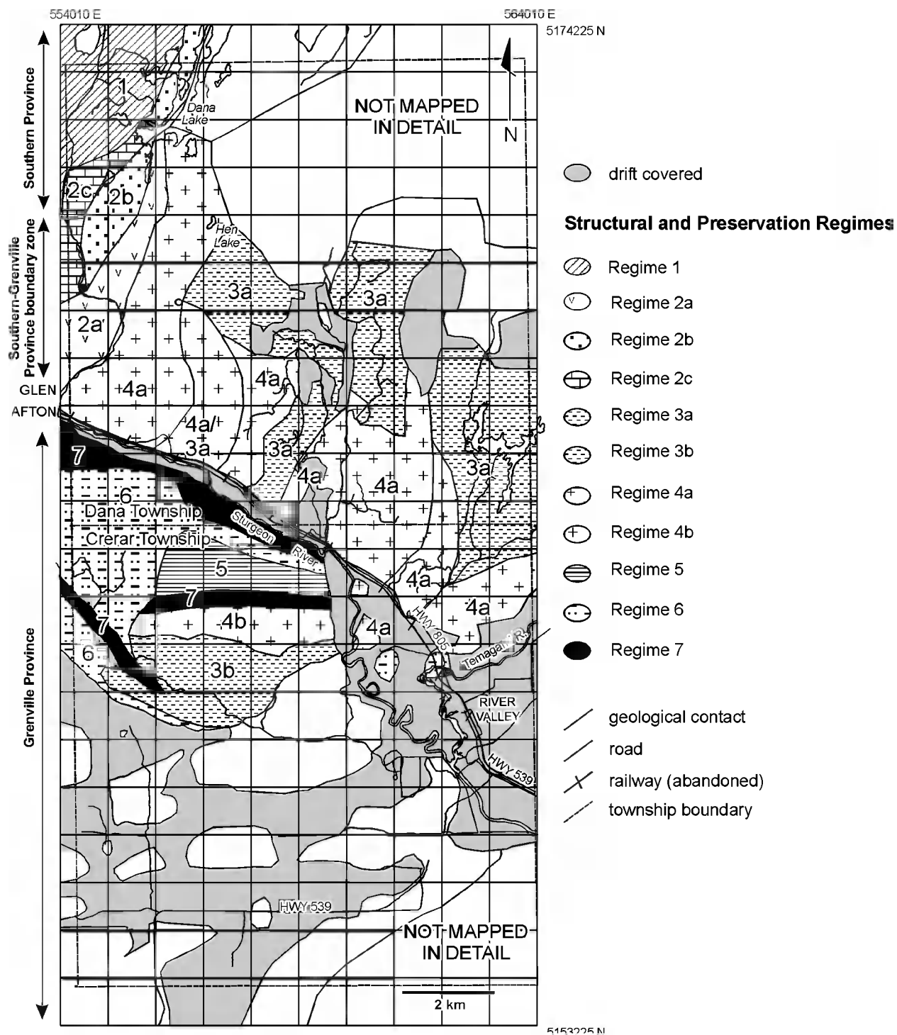
Figure 8. Map showing the degree of primary textural preservation within rocks of Crerar and Dana townships (from Easton 2003).
