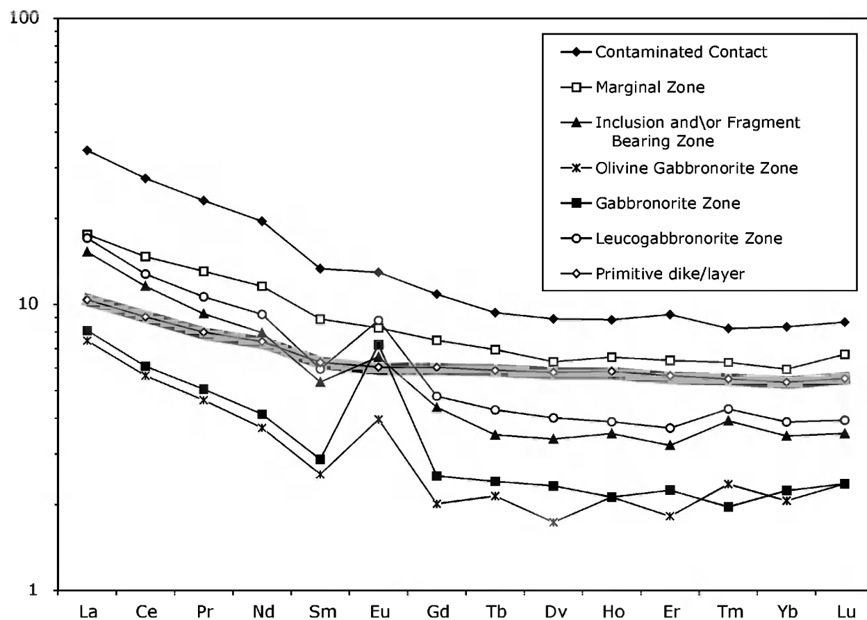
Figure 11. Chondrite-normalized rare earth element plots for the River Valley intrusion for rocks north of the Sturgeon River. Sample from the “primitive dike or layer” may represent the parent magma composition to the mineralized parts of the intrusion in Dana Township.
