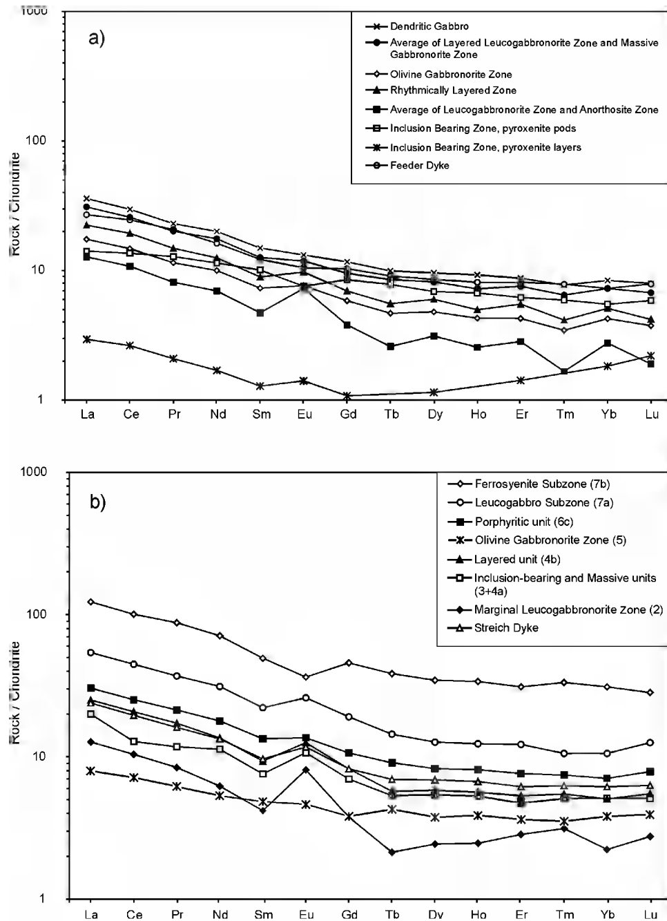
Figure 5. Chondrite-normalized rare earth element plots for the East Bull Lake and Agnew Lake intrusions. a) East Bull Lake Intrusion. b) Agnew Lake Intrusion. Data are from Peck et al. (1995) and Vogel (1996). Normalizing values are from Sun and McDonough (1989). In both diagrams, all data are the average for 2 or more samples. “Feeder dike” in Figure 5a and “Streich dike” in 5b are estimates of parent magma compositions to the East Bull Lake Intrusion and the Agnew Lake Intrusion, respectively. In 5a, note the U-shaped boninite-like pattern for pyroxenite layers from the Inclusion-Bearing Zone.
