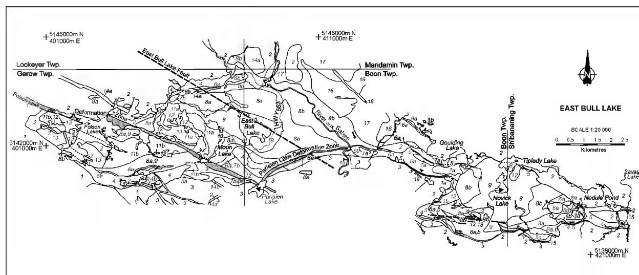
Figure 2. Geologic map of East Bull Lake Intrusion. Numbered units within the intrusion correspond to stratigraphic zones shown in Figure 3. Units 1 to 3 are Archean strata; units 14 to 17 are post-intrusion Paleoproterozoic units; for details see Peck et al. (1995).
