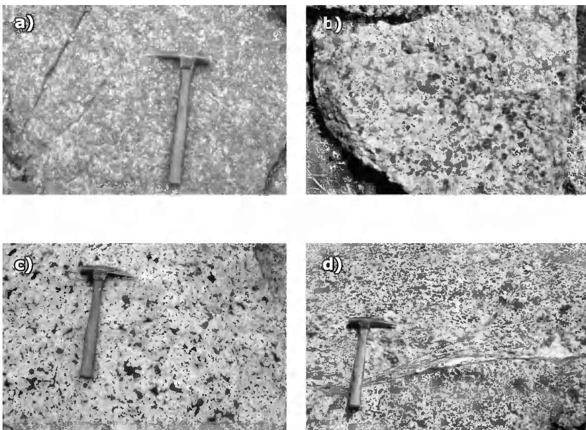
Photo 10. Progressive textural changes. a) Igneous-texture in medium-grained norite from leucogabbronorite zone of the River Valley intrusion, Crerar Township. Note dark colour of feldspars. UTM 556115E 5171466N. b) Partly recrystallized rock of the River Valley intrusion, preserving igneous-texture in medium-grained gabbronorite from leucogabbronorite zone of the River Valley intrusion, Crerar Township. Mafic minerals have thick, green-weathering amphibole coronas rimming dark orthopyroxene grains. UTM 556886E 5161009N. c) Recrystallized but massive leucogabbronorite from leucogabbronorite zone of the River Valley intrusion, Crerar Township. This rock no longer preserves primary mineralogy, but is relatively undeformed. Note white colour of feldspars, and lack of well defined crystal shapes. Mafic mineral clots are aggregates of fine-grained amphibole. UTM 557400E 5160225N. d) Typical undeformed but recrystallized leucogabbronorite from the Positano Quarry, East Bull Lake intrusive suite, Loughrin Township. UTM 547000E 5160600N. Hammer handle in all photos is 30 cm long.
