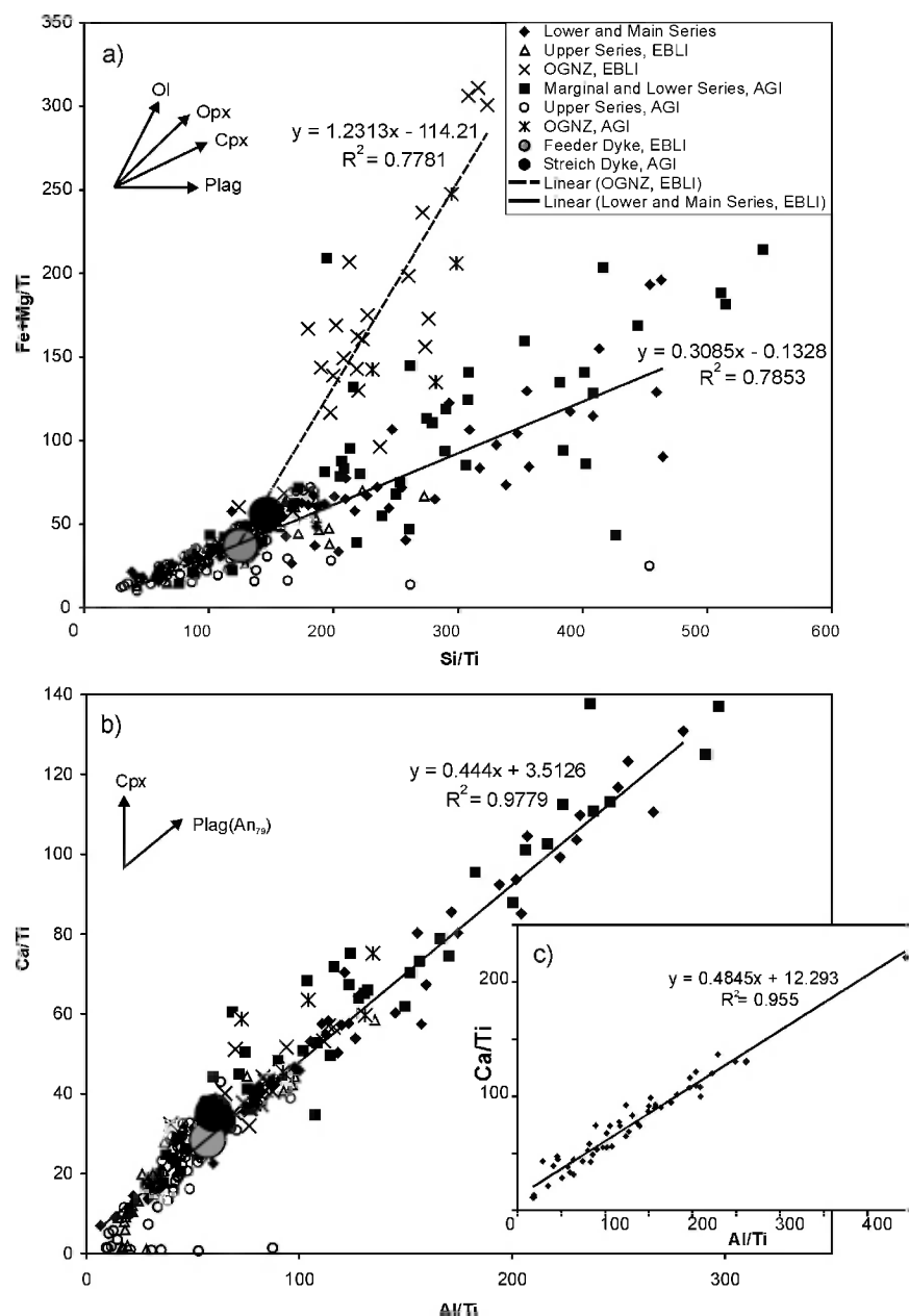
Figure 4. Pearce-element ratio diagrams for the East Bull Lake, Agnew Lake and River Valley intrusions. a) \text{Fe}+\text{Mg}/\text{Ti} versus \text{Si}/\text{Ti} plot for East Bull Lake and Agnew Lake intrusions. b) \text{Ca}/\text{Ti} versus \text{Al}/\text{Ti} plot for East Bull Lake and Agnew Lake intrusions. c) \text{Ca}/\text{Ti} versus \text{Al}/\text{Ti} plot for the River Valley intrusion. In figures 4a and 4b, solid symbols are for lower and middle portions of the stratigraphy, with open symbols for the upper part. The Olivine Gabbro-norite Zone is shown separately as are the estimated parent magma compositions for the 2 intrusions. Solid lines are fitted curves for the East Bull Lake Intrusion, as examples. Mineral vectors indicate how the data should vary if trends are due to that phase only. The data in figures 4a and 4b show that the 2 intrusions exhibit identical chemical variations. In Figure 4a, Olivine Gabbro-norite Zone rocks are clearly more mafic (primitive) in composition than the remainder of each intrusion which fall on a single trend with a much shallower (plagioclase-enriched) slope. The positions of the parent magma composition are consistent with the 2 groups being derived from cogenetic magmas. In Figure 4b, data for all samples fall on a linear trend with a slope in the range 0.40 to 0.45 indicating that calcic plagioclase feldspar mainly controls this trend, and that clinopyroxene is not a major modal phase in these rocks. In the lower left of 4a, samples of Upper Series rocks deviate from the trend near the origin of the diagram because they have primocryst ilmenomagnetite and thereby, Ti is no longer a conserved element. In figure 4c, rocks from the River Valley intrusion display a similar plagioclase-controlled trend, but with a greater proportion of samples lying closer to the origin, reflecting a slightly more mafic bulk composition of the samples.
