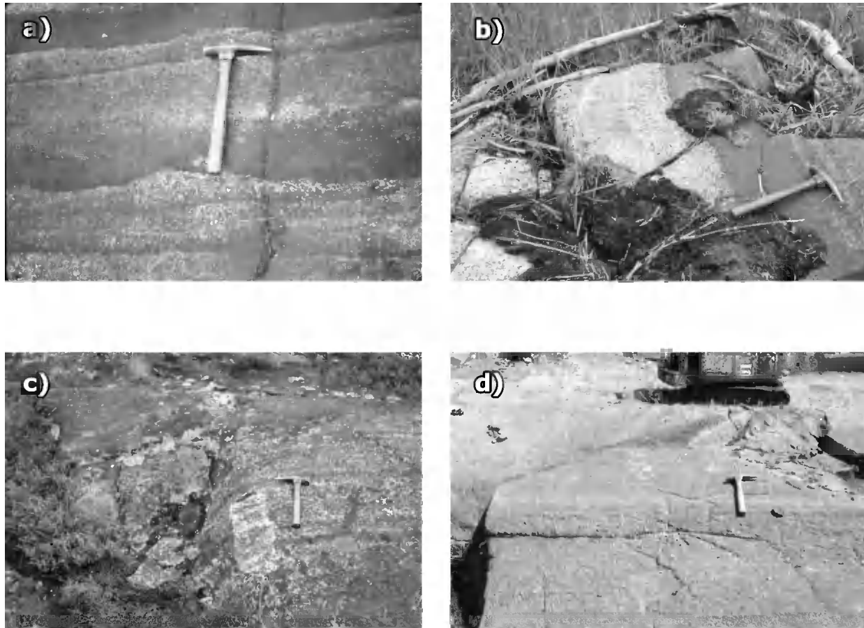
Photo 11. a) Igneous layering within the norite zone, River Valley intrusion, Crerar Township. UTM 556769E 5159980N. b) Igneous layering within the River Valley intrusion in Crerar Township, near the top of the anorthosite zone and the base of the olivine gabbro-norite zone. Dark layers are melanorites, some of which are olivine-bearing. UTM 557390E 5160360N. c) Layering within leucogabbro-noritic rocks immediately above the heterogeneous basal zone of River Valley intrusion, Crerar Township. UTM 557585E 5159590N. d) Large-scale igneous layering within leucogabbro-noritic rocks of the River Valley intrusion exposed in the Dana Quarry, Dana Township. UTM 558630E 5165385N. Hammer handle in all photos is 30 cm long.
