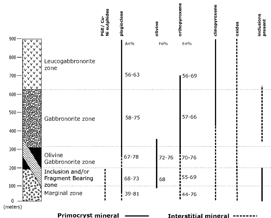
Figure 9. Interpreted stratigraphic sequence and distribution of primary mineral phases and compositions within the River Valley intrusion north of the Sturgeon River. From Easton (2003).
