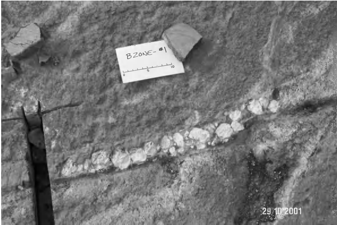
Photo 9. Diabase dike containing large, rounded plagioclase crystals, similar to the nodules of the Nodular Anorthosite unit, cutting across rocks of the Inclusion-Bearing Gabbronorite Zone, Lower Series, of the Agnew Lake Intrusion.
