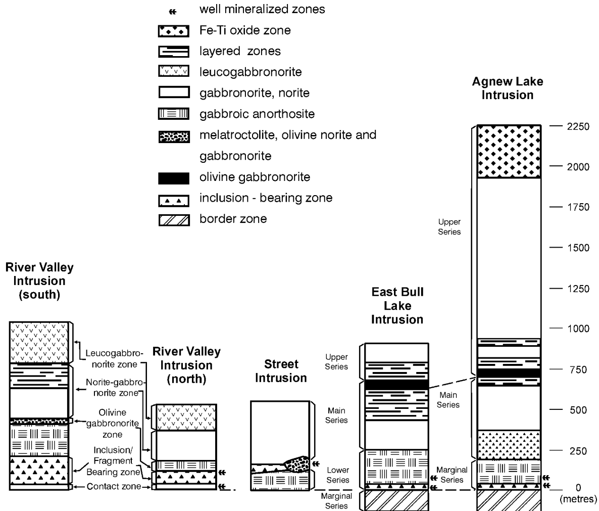
Figure 10. Generalized cross-sections for the Street metagabbro and the River Valley, East Bull Lake and Agnew Lake intrusions of the East Bull Lake intrusive suite. East Bull Lake section modified from Peck et al. (1995), Agnew Lake Intrusion section modified from Vogel (1996), River Valley data from Easton (2003).
